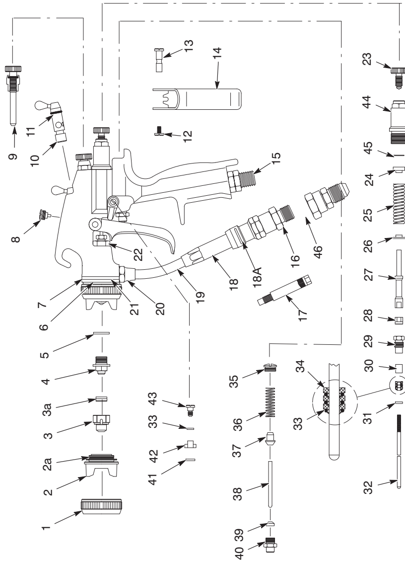
Figure 4 Trilogy AAA Spray Gun Parts
